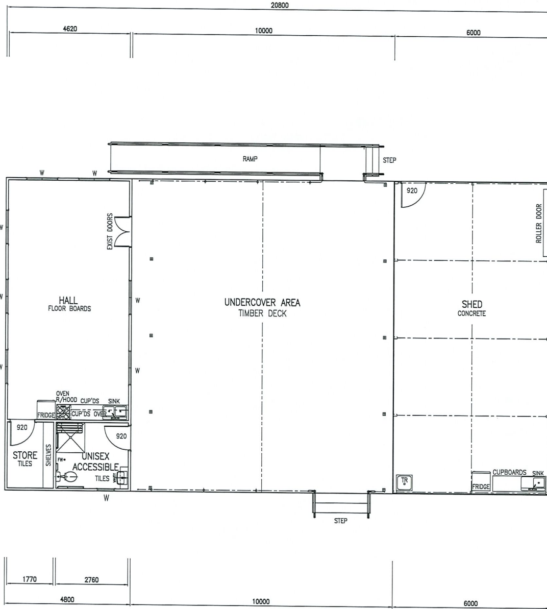
FLOOR PLAN 1:50 -OPTION 1
