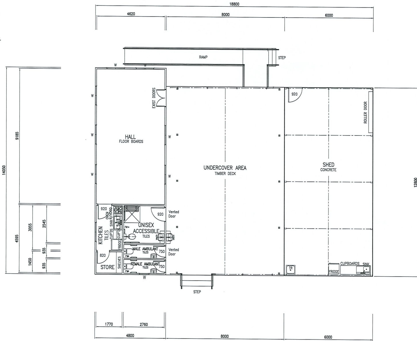
FLOOR PLAN 1:50 -OPTION 2
